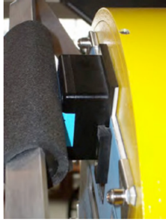
Figure 4 Proper Orientation of Infrared Sensor on GeoGauge
