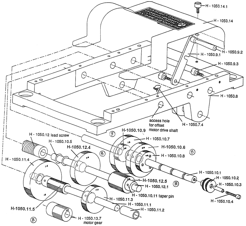
Gear Housing Frame, H-1050.8
