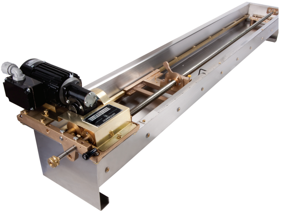
Ductility Machine
